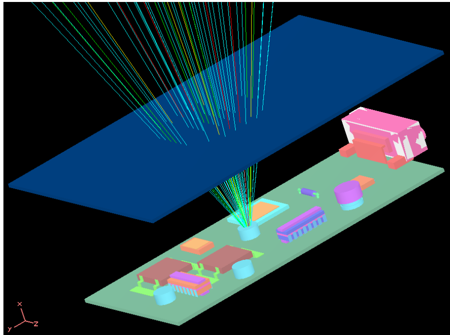
Fig. 3. Post processing of a ray tracing calculation. The directions of critical rays are clearly identified.
